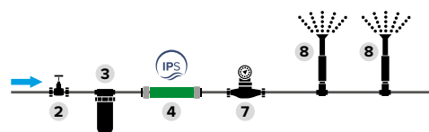
D INSTALLATION IN THE IRRIGATION SYSTEMS
